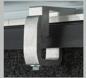
Clamp installation, no drilling required.
